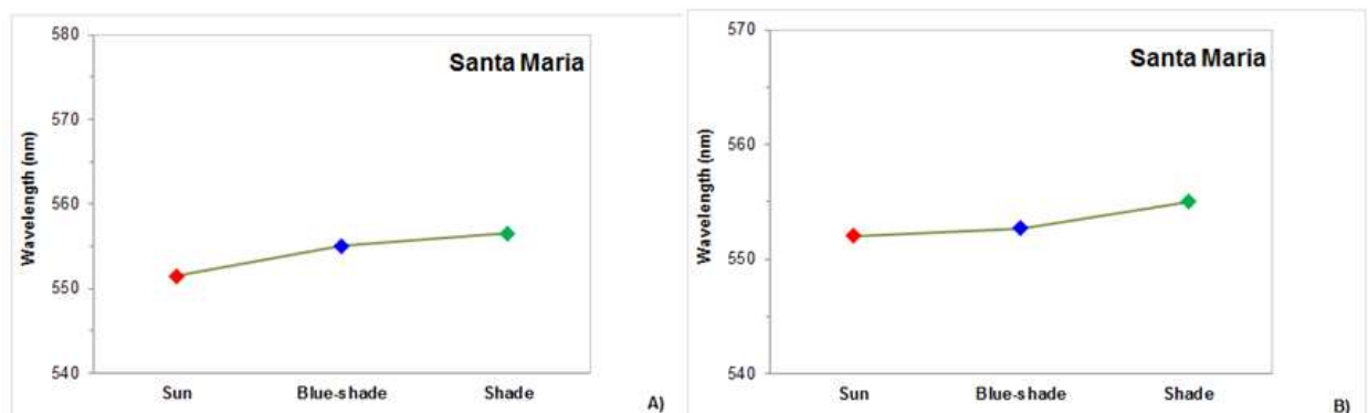
Figure 7. Values of the "dominant" wavelength, of the sun, blue-shade and shade type leaves; of Santa Maria (pear) variety; A) Area under water, B) Area above water.
